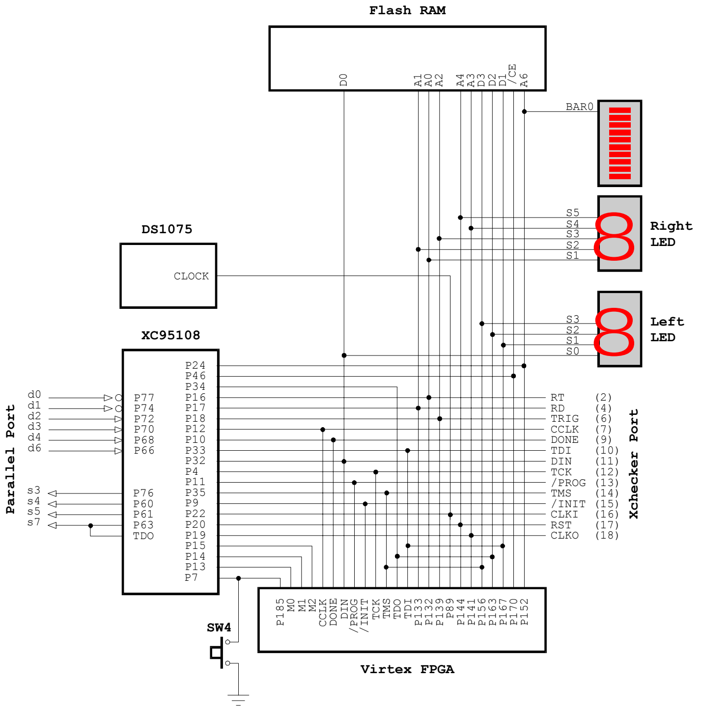
Figure 2: XSV Board CPLD connections.
